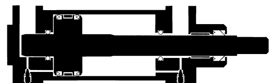
Non-magnetic piston
